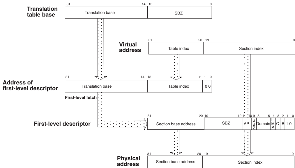
Figure 3-3 Section translation
